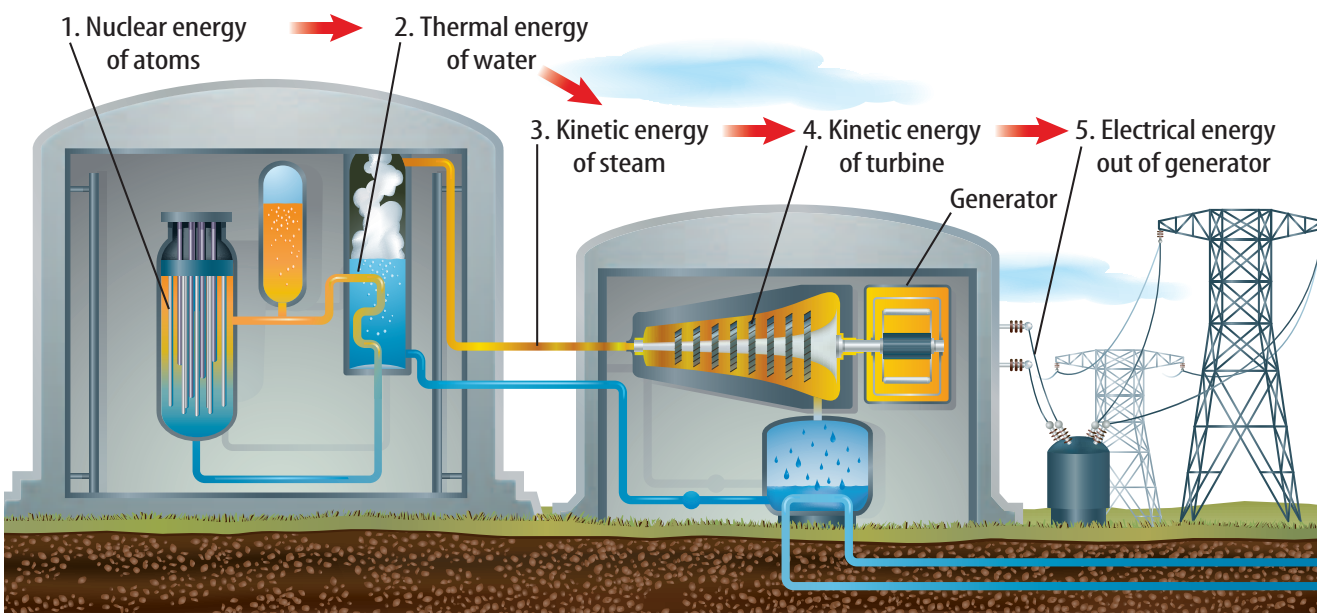
Figure 18 To obtain electrical energy from nuclear energy, a series of energy transformations must occur.
